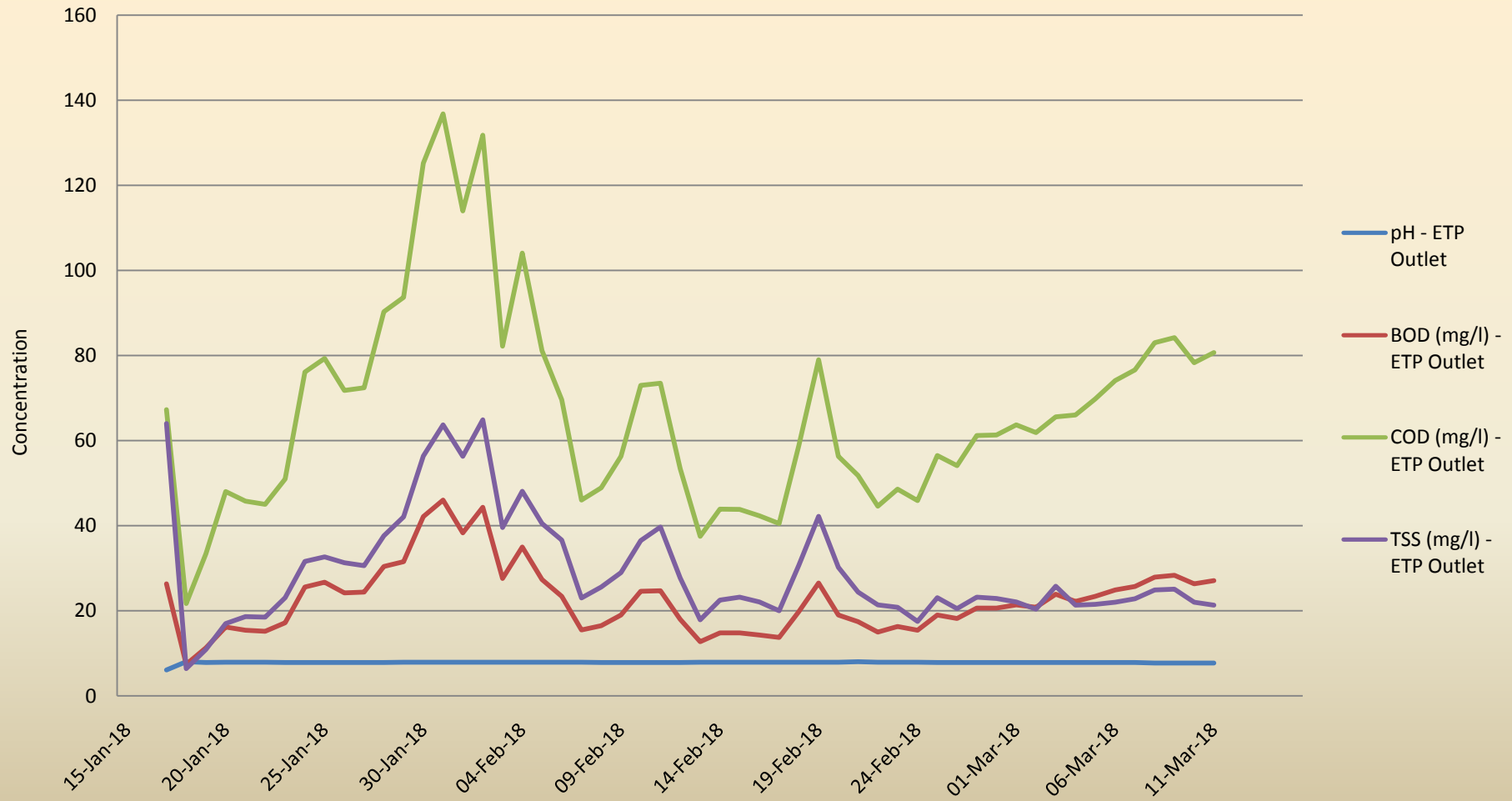
Effluent Trend (2017-18) in M/s. Krishak Sahakari Shakkar Karkhana Mydt., Dist. Guna (M.P.)
