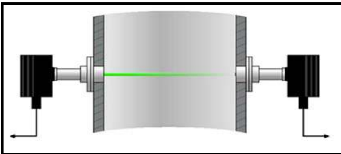
Figure 5.1 : Light Attenuation
