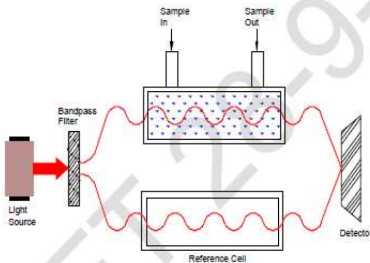
Figure 5.2 : NDIR System
