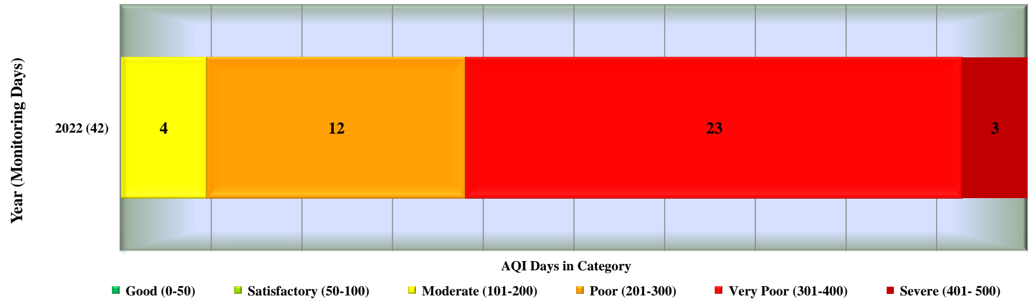
Days in various AQI categories of Gwalior, DD Nagar (Year - 2022)
